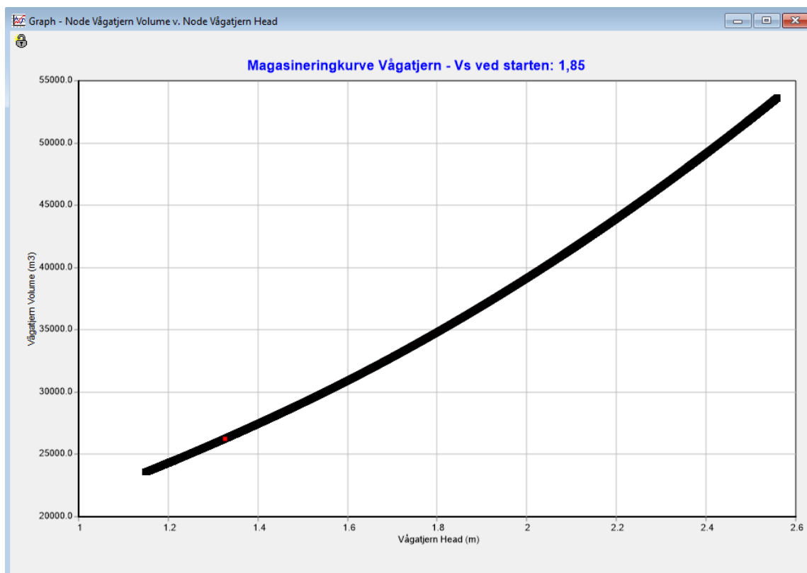
Figur 6: Magasinkurve for Vågatjøerna
